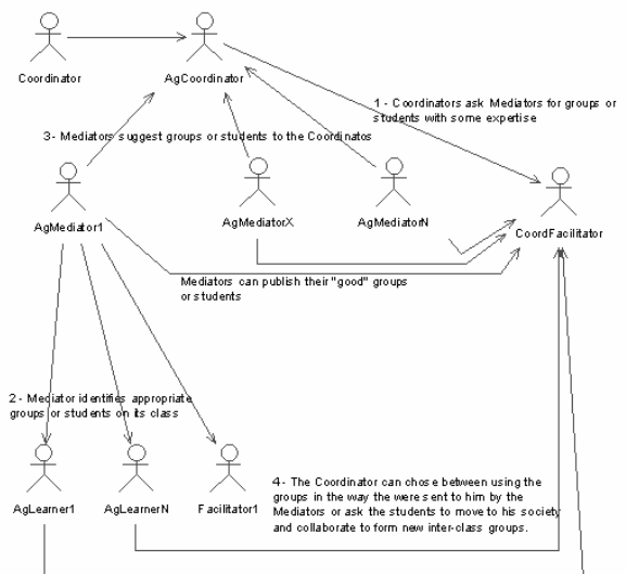
Figure 1 - Group formation using software agents
