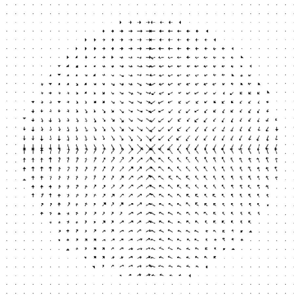
Figure 4: Example of estimated velocity provided by Horn-Shunck method
