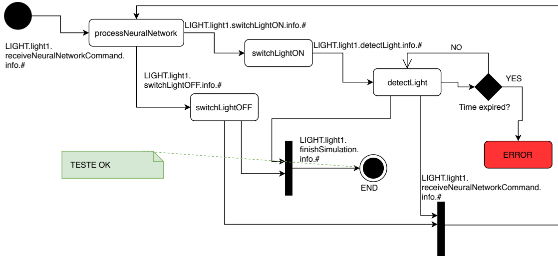
Figure 10: Simplified state machine for verifying test cases generated for the functions “switch the light ON” and “switch the light OFF”.
