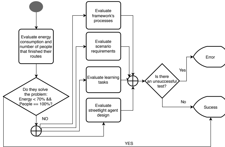
Figure 4: Testing steps.
