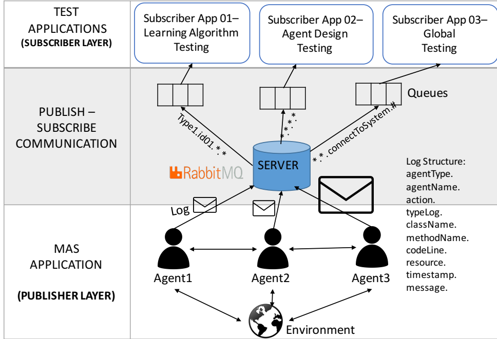
Figure 5: A Publish-Subscribe-based architecture to test MASs.
