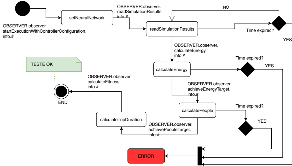
Figure 9: Simplified state machine for verifying test cases generated for the function “evaluate selected solution”.
