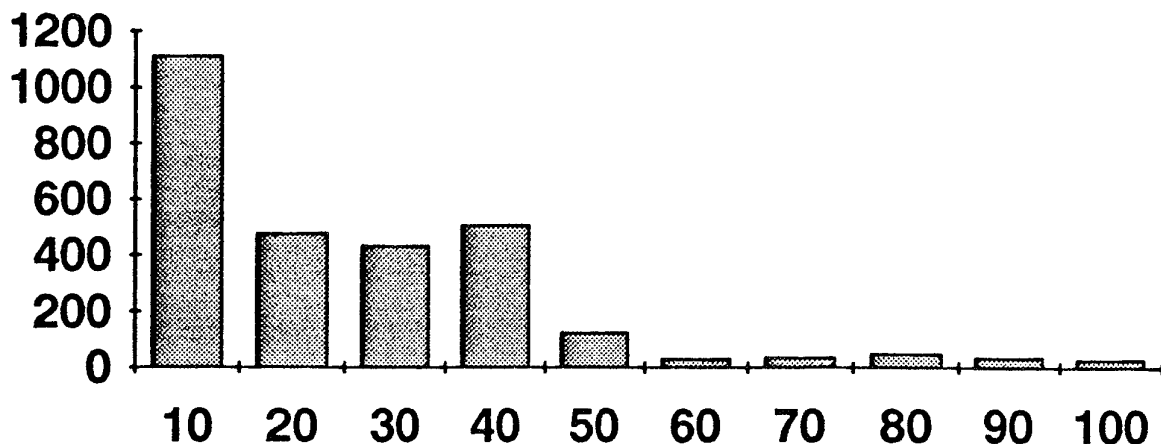
Figure 4: Sensitivity of the secondary criterion with respect to the maximum accepted level of deterioration (in percent) of the primary criterion
